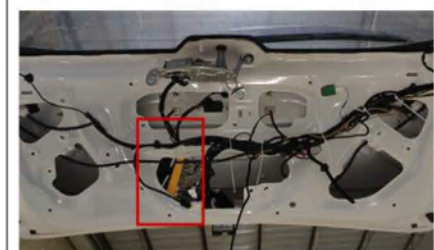
27. Connect the control box harness and fix the control box
