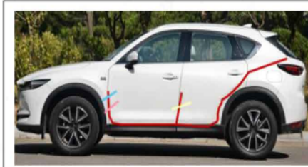
25. Threading diagram (blue: power cord, pink: front button line, yellow: unlock signal line)
